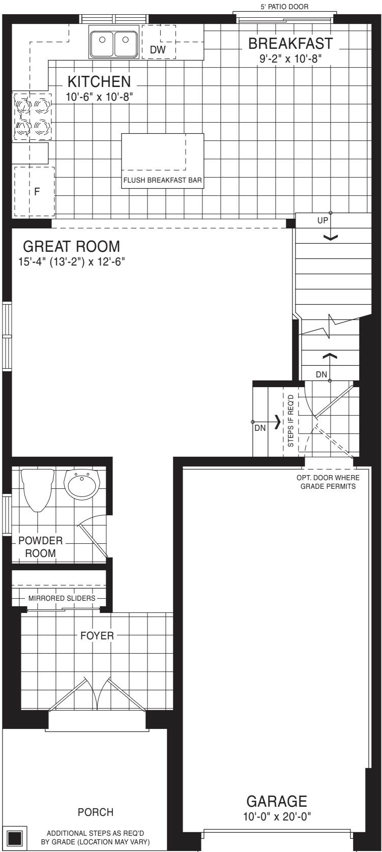
MAIN FLOOR PLAN STYLE A
