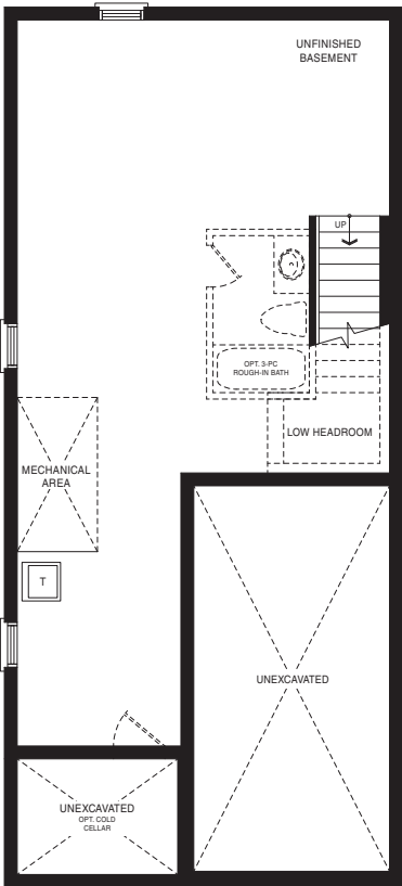
BASEMENT PLAN STYLE A
